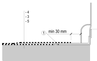
2.2. b Connection detail of foil from asphalt strips
