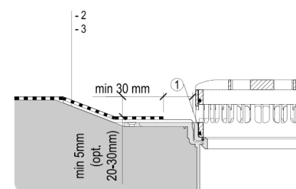
3.2.a mPVC foil connection detail (TPO-FPO)
