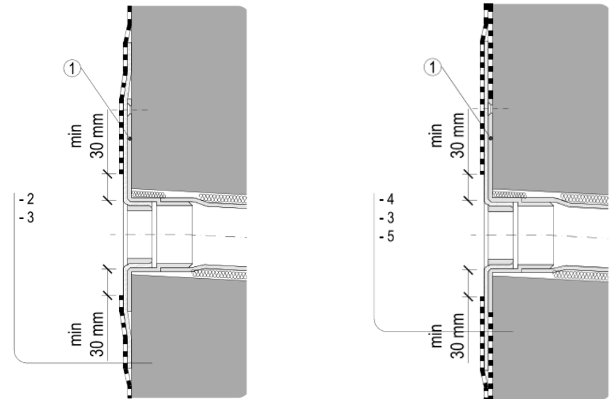
2.2.a Detail - mPVC-verbindungsfolie (TPO-FPO)
