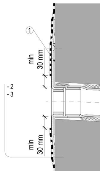
2.2.a mPVC foil connection detail (TPO-FPO)
