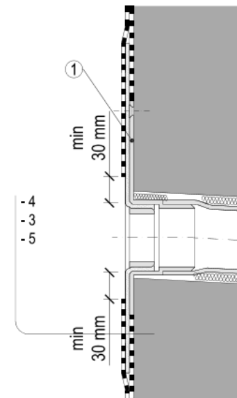
2.2.b Connection detail of foil from asphalt strips
