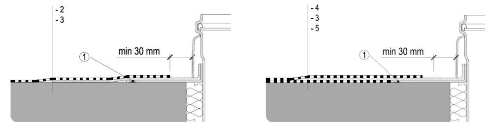
2.2.a Detail - mPVC-Verbindungsfolie (TPO-FPO)
