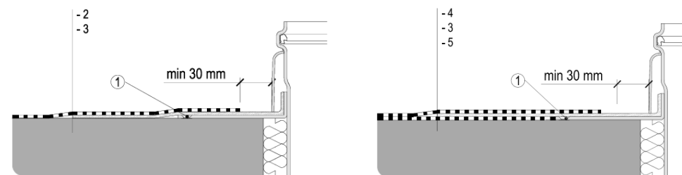
2.2.a mPVC foil connection detail (TPO-FPO)
