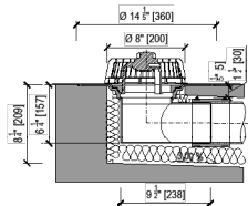
horizontal roof drain DN 4
